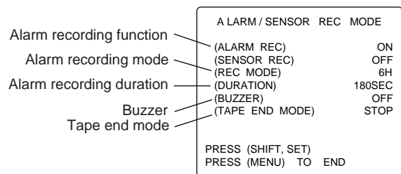
Alarm/sensor recording mode setting screen
